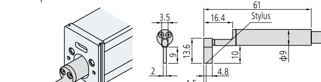
Deep Groove Detectors
