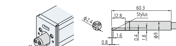
Extra Small Hole Detectors
