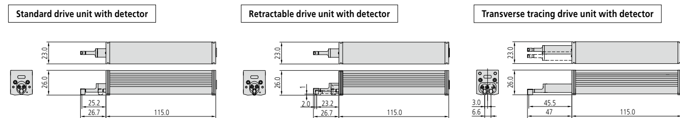
Drive unit attached with detector
