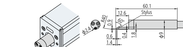
Gear-tooth Surface Detectors
