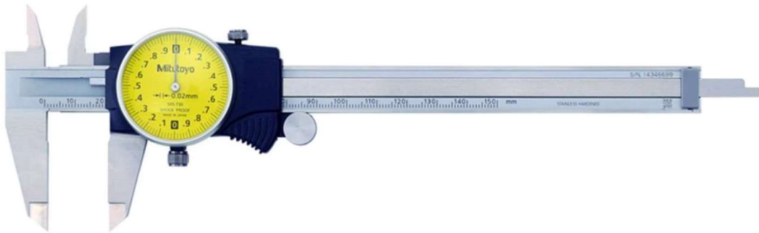
Dial Caliper (Graduation: 0.02mm, 2 mm per revolution)
